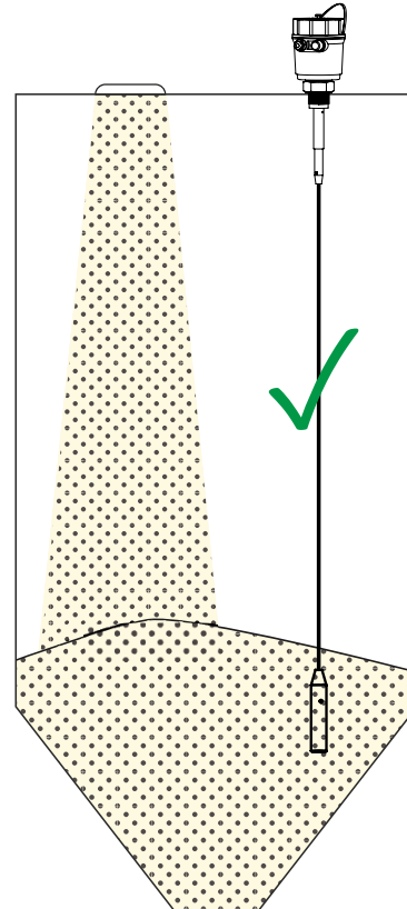
Figure 6 - Correct Installation
